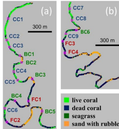
Fig. 4. Target areas (west reef slopes) of Barrang Lompo (a) and Bone Batang (b) extracted from Fig. 3. Small squares with labels indicate the locations of fish survey sites (20 m \times 20 m) of continuous coral reefs (CC), boundary of coral reefs (BC) and few coral reefs (FC)
